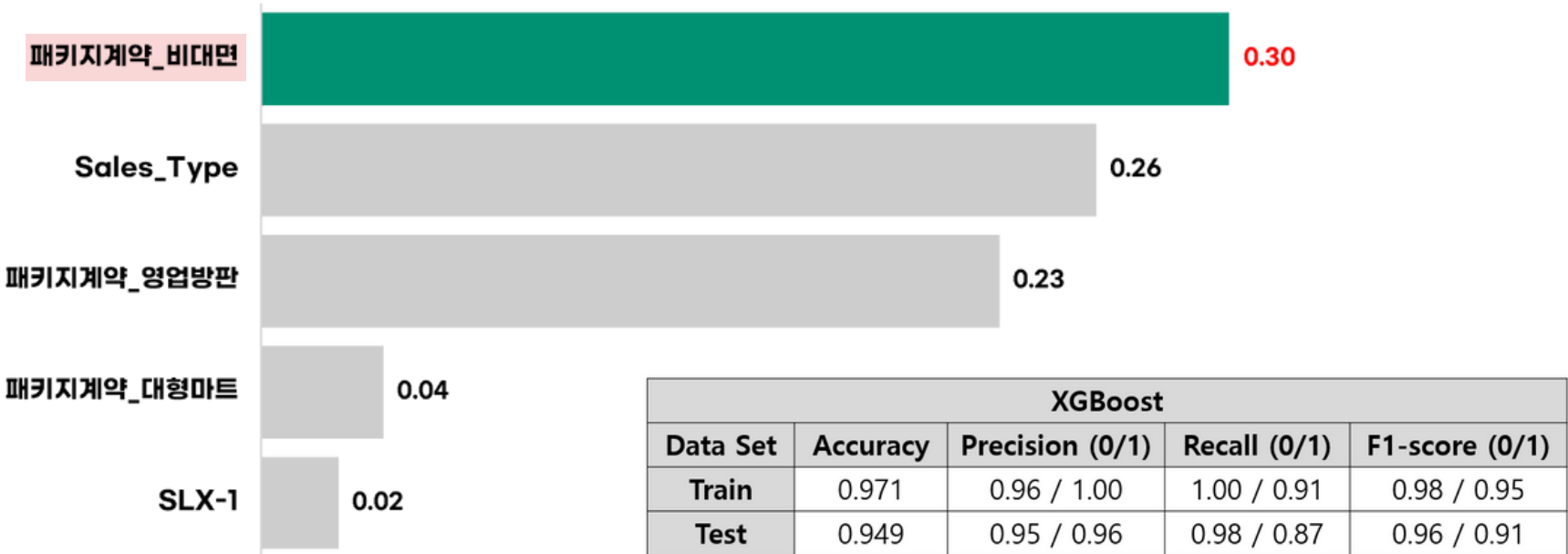
[XGBoost]
